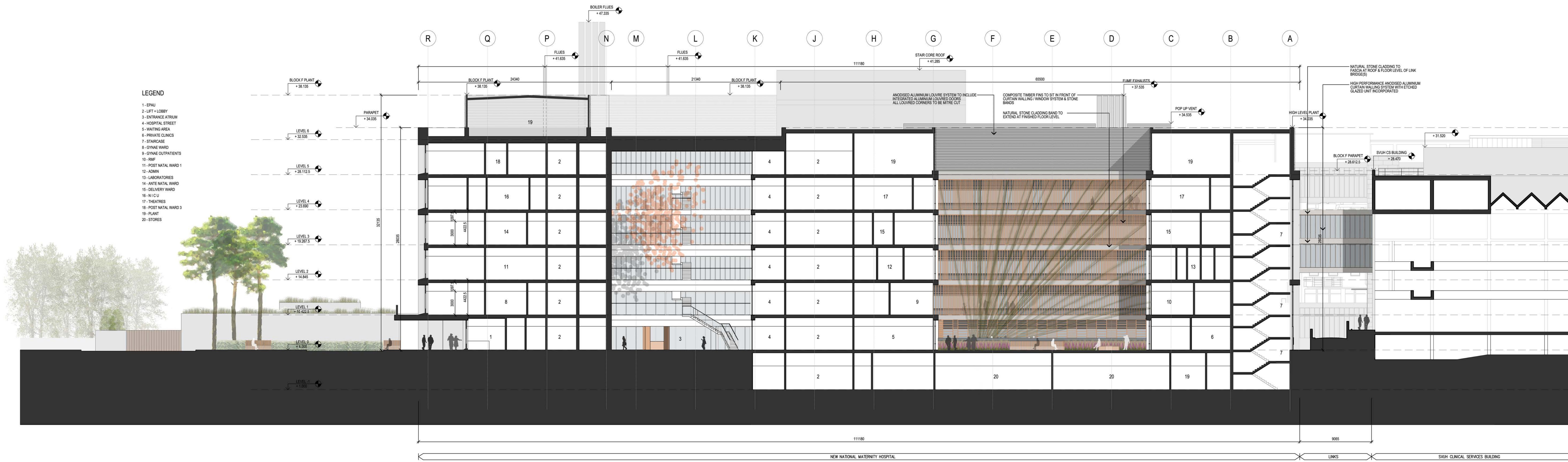
PROPOSED SECTION E-E SCALE 1:200
