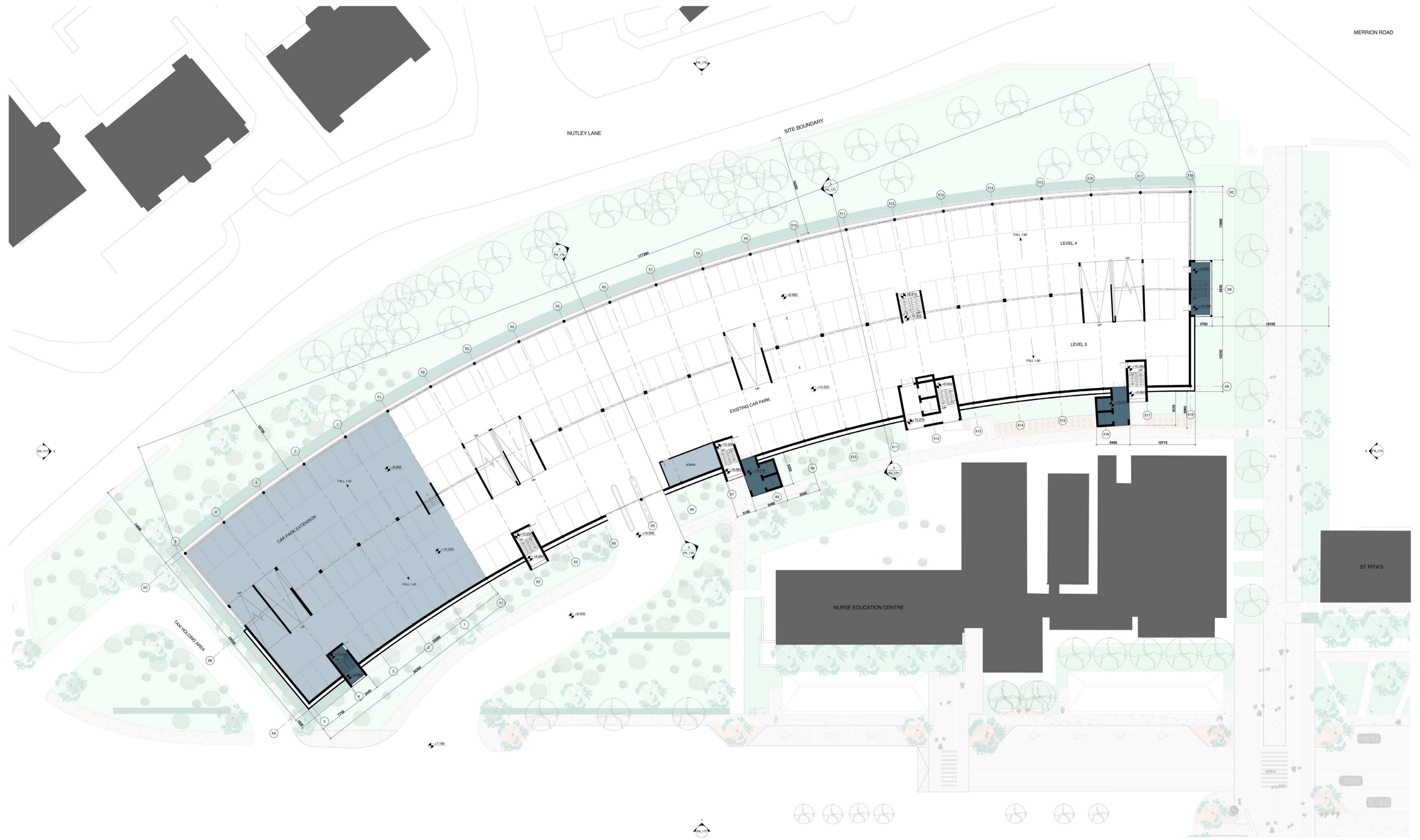
1 PROPOSED CAR PARK LEVEL 4 & 5 PLAN SCALE 1:200
